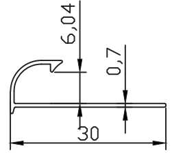
FC-5349 0.092 kg/m
