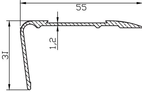
MB-9920 0.349 kg/m
