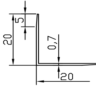
FC-10487 0.070 kg/m
