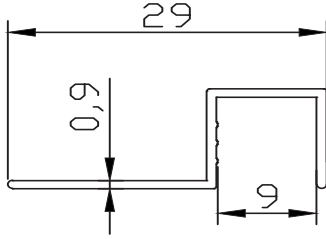
FC-10010 0.119 kg/m
