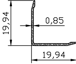
FC-10412 0.087kg/m
