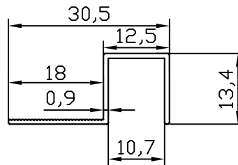
FC-10421 0.133kg/m
