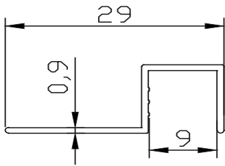
FC-10010 0.119 kg/m
