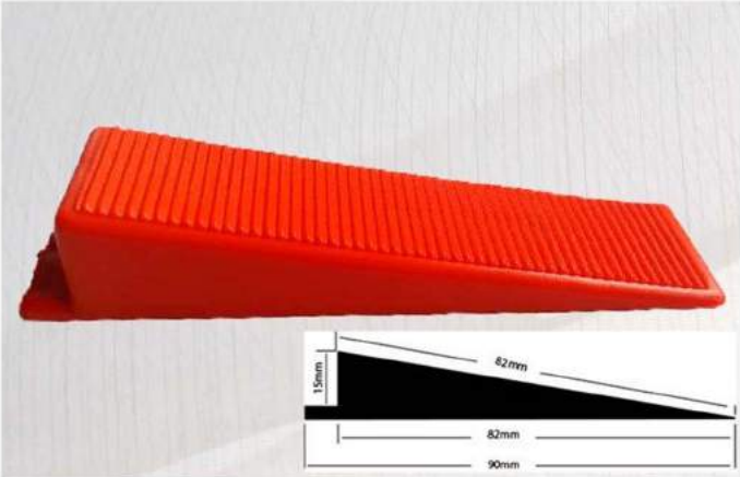
Seviye Tespit Takozu Levelling System Wedges
