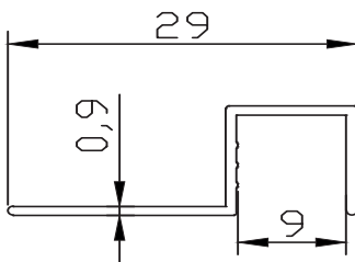
FC-10010 0.119 kg/m
