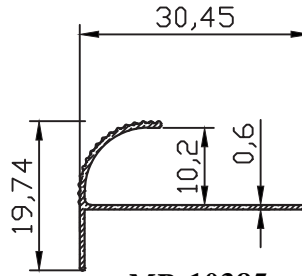
MB-10385 0.98 kg/m
