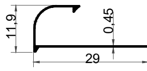
KF-1085 0.065kg/m
