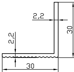
MB-9052 0.324 kg/m
