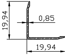
FC-10412 0.087kg/m
