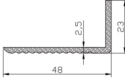
MB-9026 0.430 kg/m
