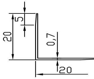
FC-10487 0.070 kg/m
