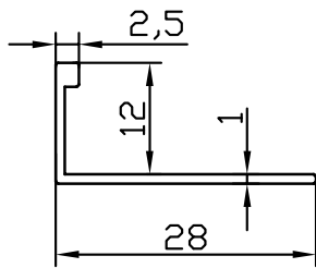
FC-10497 0.119 kg/m
