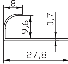
FC-10015 0.081 kg/m
