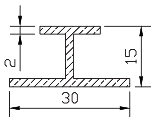
PR-9094 0.303 kg/m
