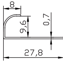
FC-10015 0.081 kg/m
