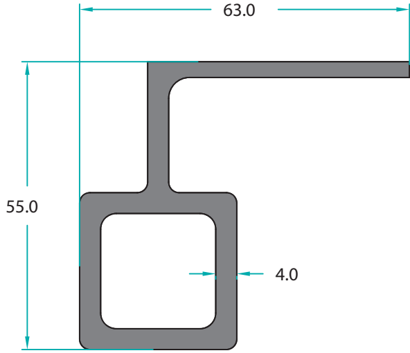
MO-11207 1,799 Kg/m
