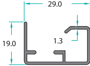
MO-13741 1,016 Kg/m
