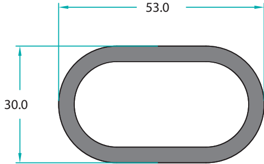
MO-11220 1,385 Kg/m
