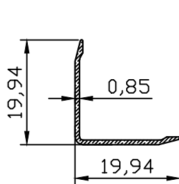
FC-10412 0.087kg/m
