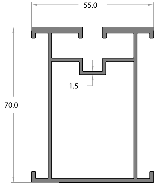
GE-13798 1,390 Kg/m
